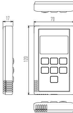
SIMPLIFIED REMOTE CONTROLLER (CZ-RE2C2)
