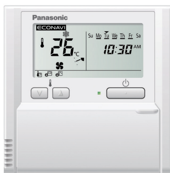
Dimensions H 120 x W 120 x D 20 mm
